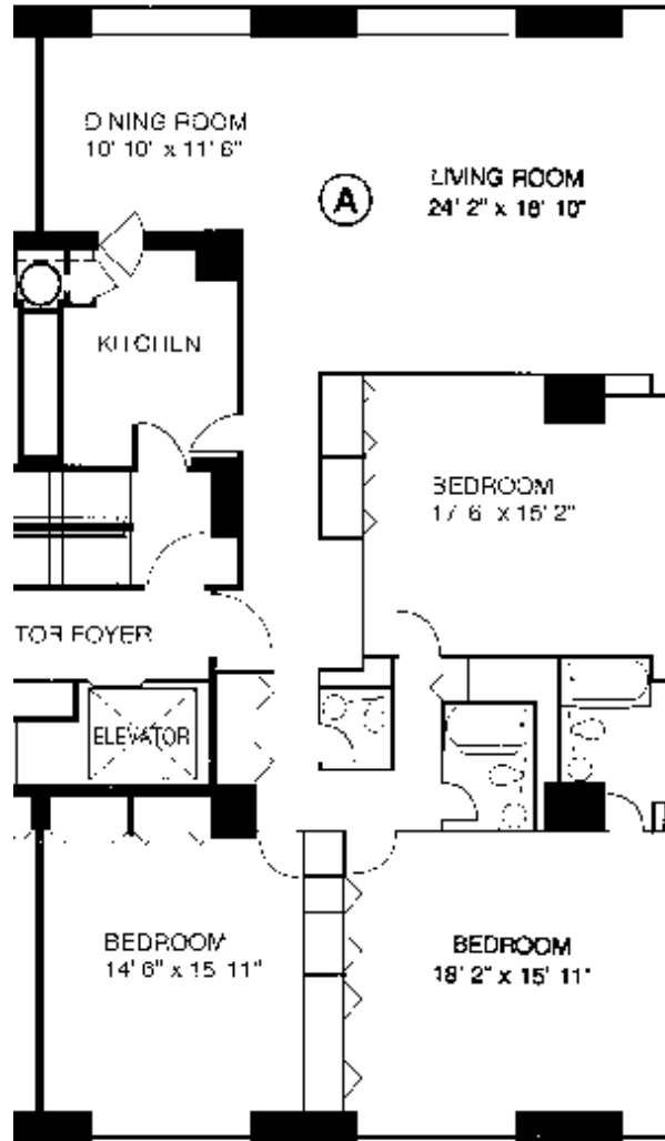
Floorplan A 3BR 2.5BA 2,200 SF
